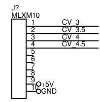
0 TO 5V CONTROL VOLTAGES SIX 10K FRONT PANEL POTS WITH SWITCHED JACK INPUTS
